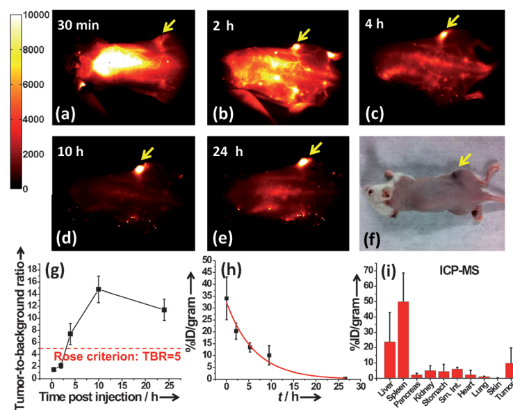
Figure 3. NIR-II fluorescence imaging of a xenograft 4T1 tumor with high uptake of 6PEG-Ag 2 S QDs. (a–e) Time course of NIR-II fluorescence images of the same mouse injected with 6PEG-Ag 2 S QDs in Figure 2. These results were reproduced with a total of three mice. f) A white-light optical image of the same mouse at 24 h p.i. The tumor mass was visibly darkened owing to high uptake of 6PEG-Ag 2 S QDs. g) The tumor-to-background ratio (TBR) plotted as a function of time p.i. for NIR-II images, indicating a 100% certainty of the tumor being identified from the NIR-II image after 4 h p.i., according to the Rose criterion. h) A representative plot of the % ID/gram of the 6PEG-Ag 2 S QDs in the blood versus time after tail-vein injection, as determined by the NIR-II fluorescence of the blood samples. A first-order exponential fits the data points with a half-life of circulation for the 6PEG-Ag 2 S QDs of 4.37 \pm 0.75 h. This half-life measurement was repeated with two other mice ( 3.98 \pm 1.16 h and 3.51 \pm 0.86 h, see Figure S5). i) Quantitative biodistribution of 6PEG-Ag 2 S QDs in various organs and the tumor 72 h after injection based on ICP-MS.
